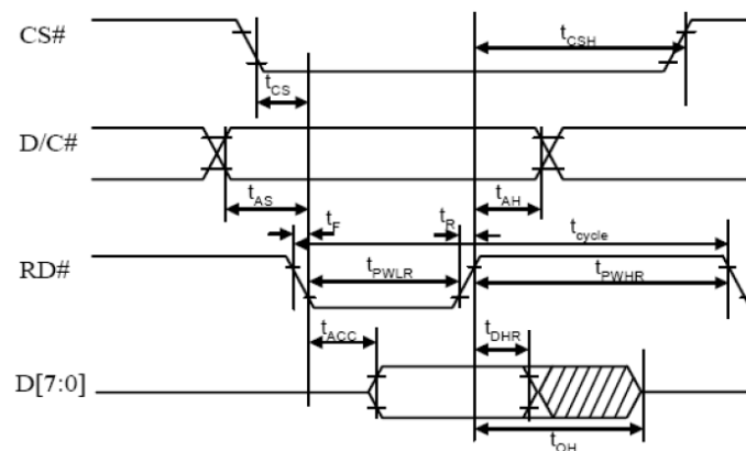
Read Timing
