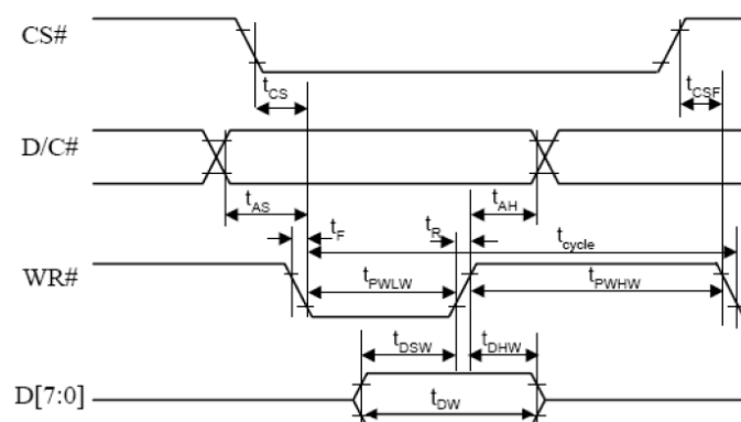
Write Timing
